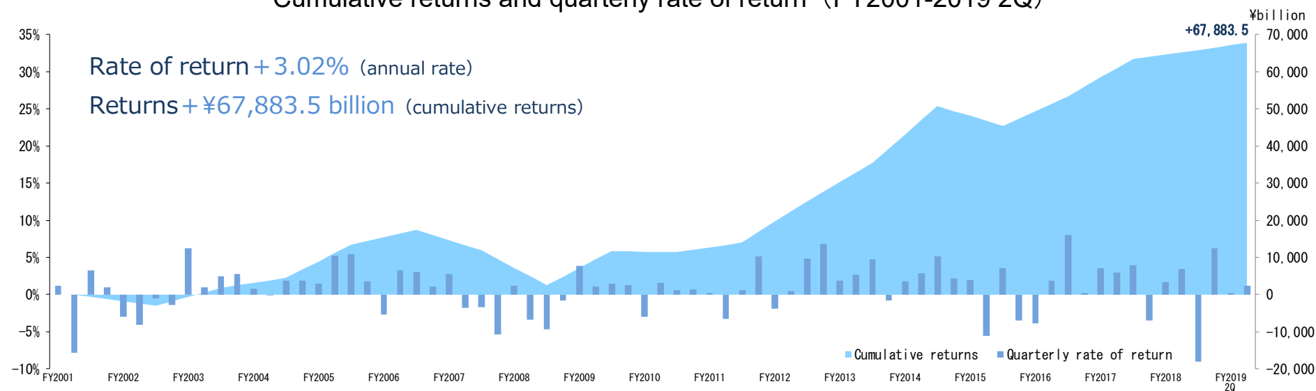
Cumulative returns and quarterly rate of return (FY2001-2019 2Q)
